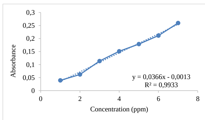
Fig. 2. Iron (Fe) standard calibration curve
