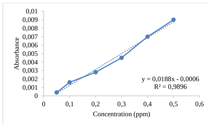
Fig. 3. Lead (Pb) standard calibration curve
